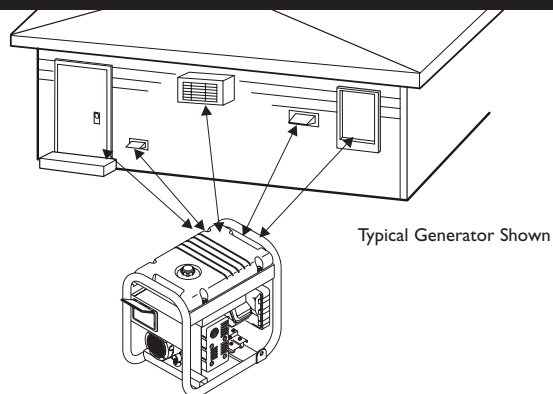
Figure 3 — Generator Clearance
